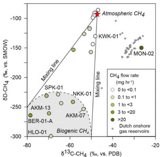
Fig. 6. Carbon and hydrogen isotopic composition of methane in samples collected after completion of static chamber measurements at 1 m depth. Grey dots show isotopic composition of samples taken from onshore Dutch gas reservoirs (NLOG, 2018). Isotopic composition of northern-hemisphere atmospheric methane based on Rice et al. (2016).
